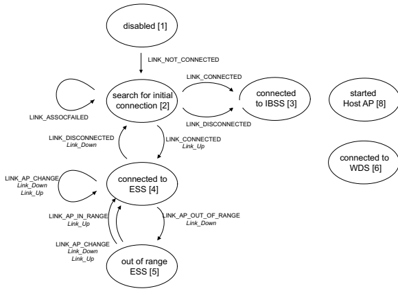
Figure 4: How Prism2 firmware states map to the link_up and link_down trigger.
