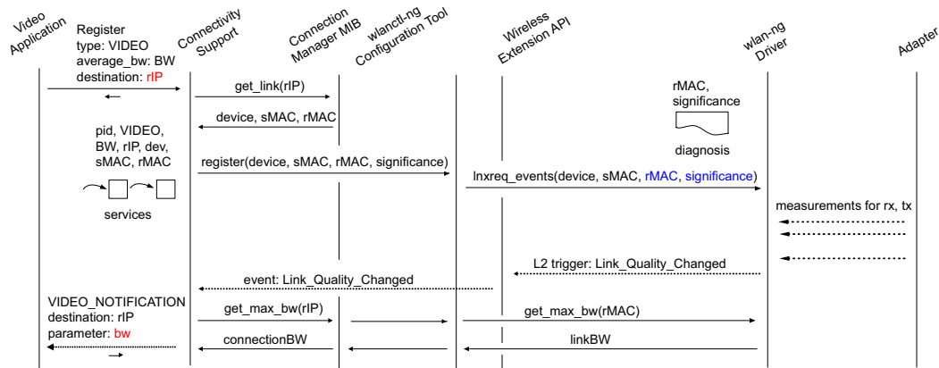
Figure 5: MSC for the example of a varying link quality.
