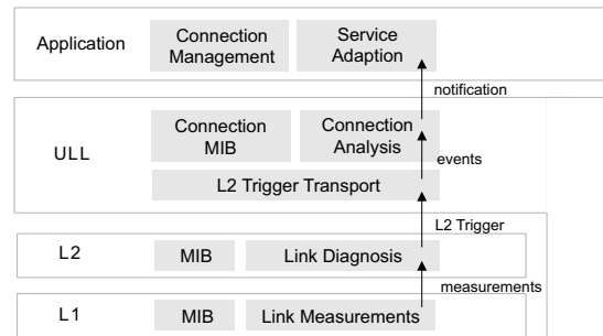
Figure 1: Notification Hierarchy using unified L2 triggers. Here ULL stands for Unified Link Layer.
