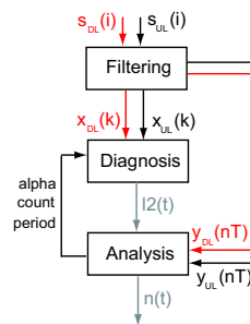
Figure 2: Model of the signal flow for uplink (UL) and downlink (DL) direction. Here following notation is used: s - measurement samples, x, y - link layer metrics, l2 - discrete L2 trigger, n - application notifications.
