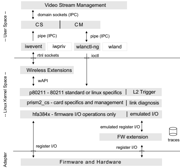
Figure 3: Overall Implementation Architecture of Linux testbed.
