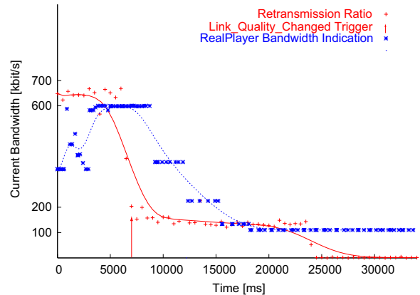
Figure 8: Timing advance for ASM with L2 trigger based on RR.
